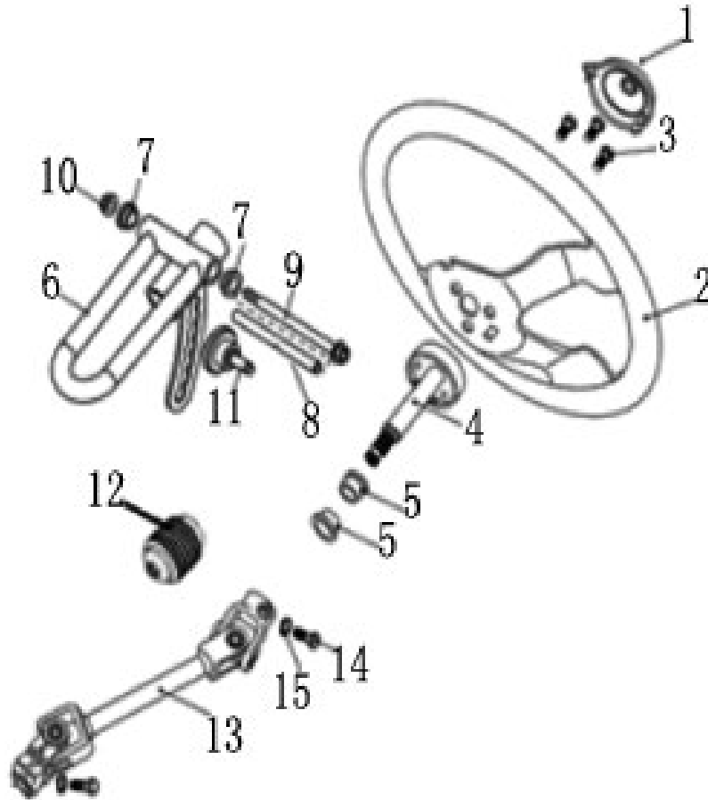
FIG. 25 STEERING WHEEL
