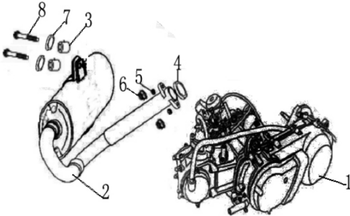
FIG. 29 ENGINE & EXHAUST
